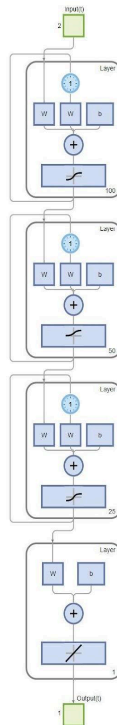
Fig. 12: Proposed RNN structure
