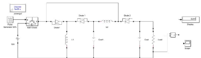
Fig. 9: MATLAB\Simulink of 50% Duty Pulse Generator
